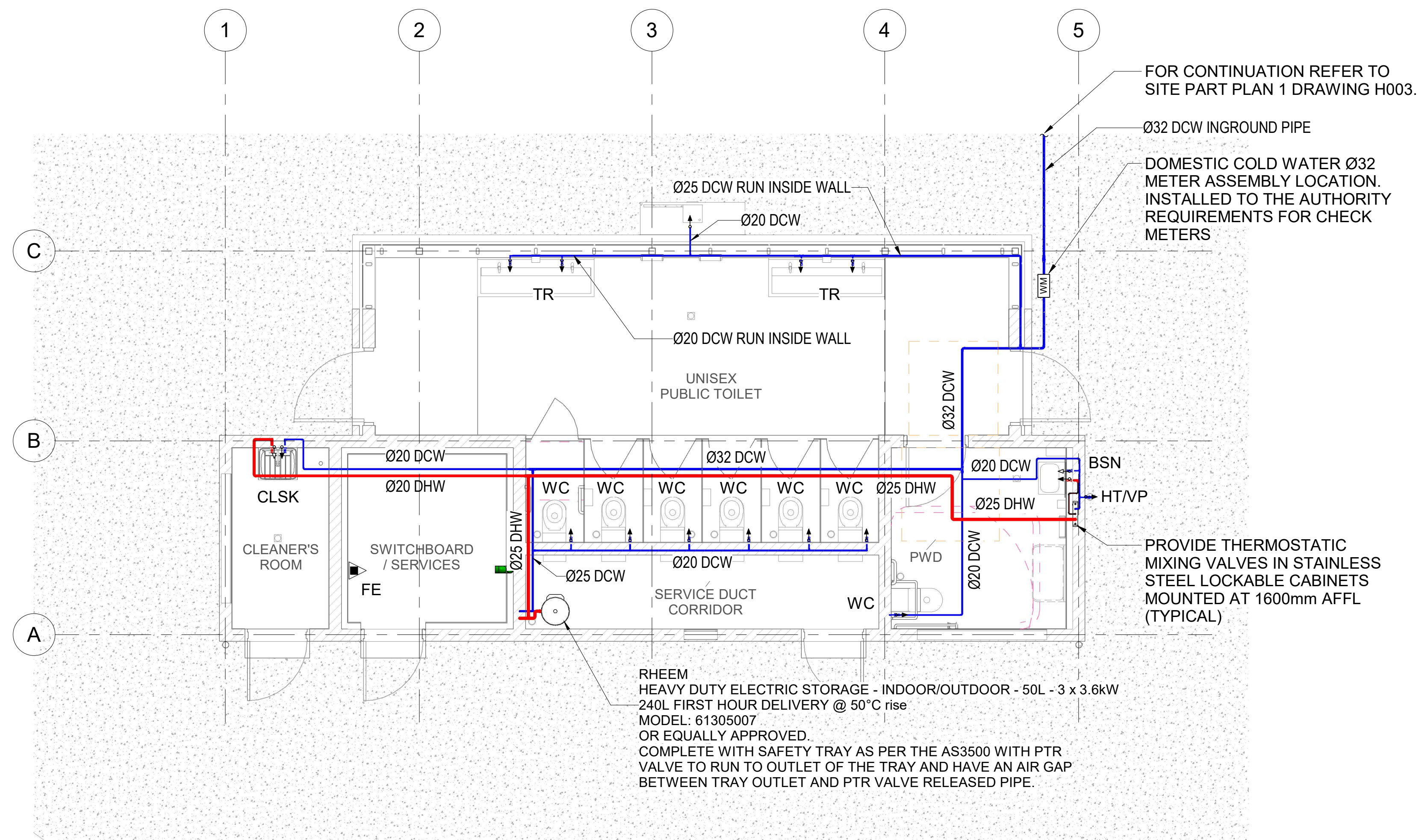
GROUND FLOOR WATER RETICULATION LAYOUT
